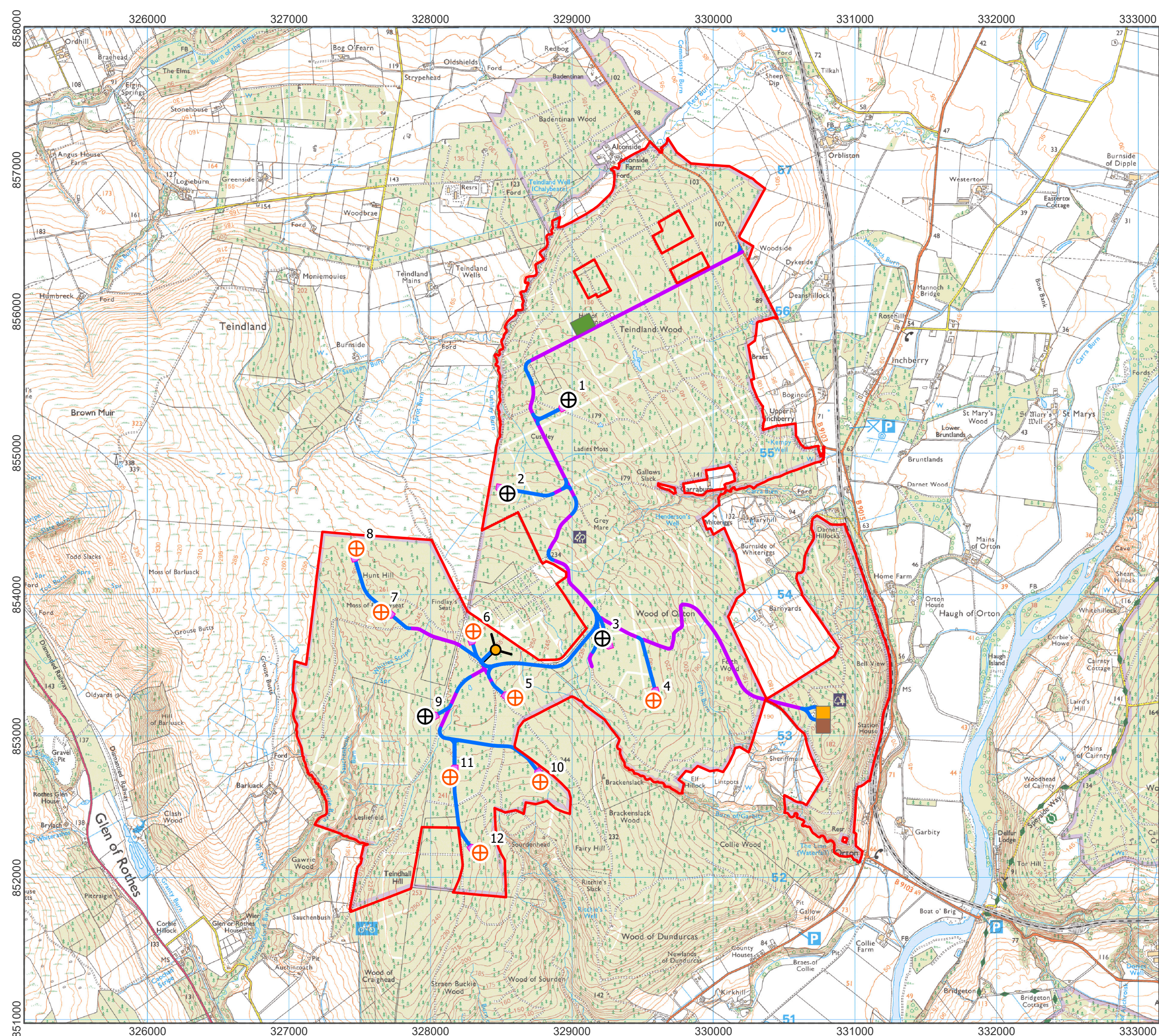
Figure 4.1 - Site Layout
