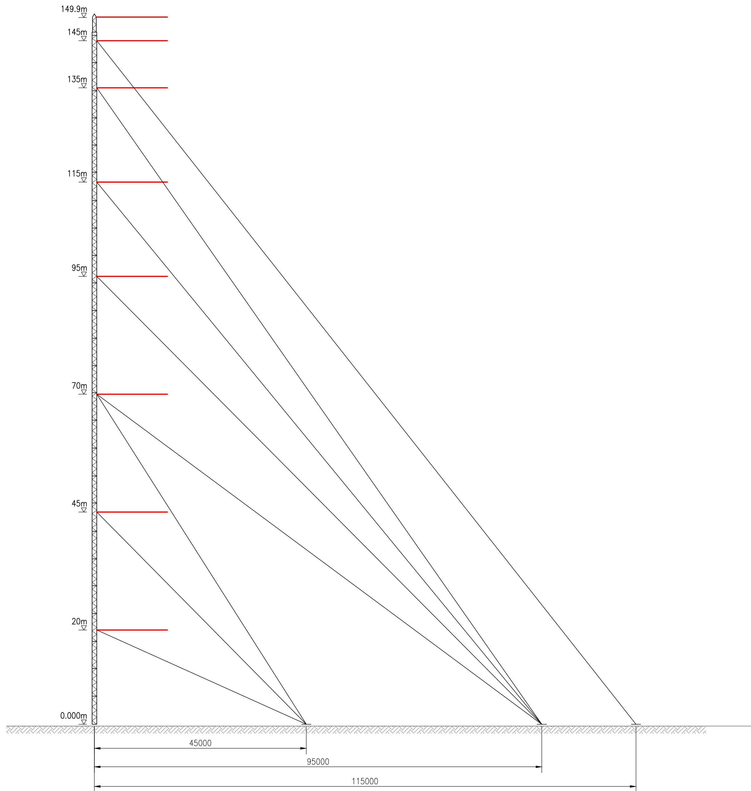
METEOROLOGICAL MAST ELEVATION (SCALE 1:500)
