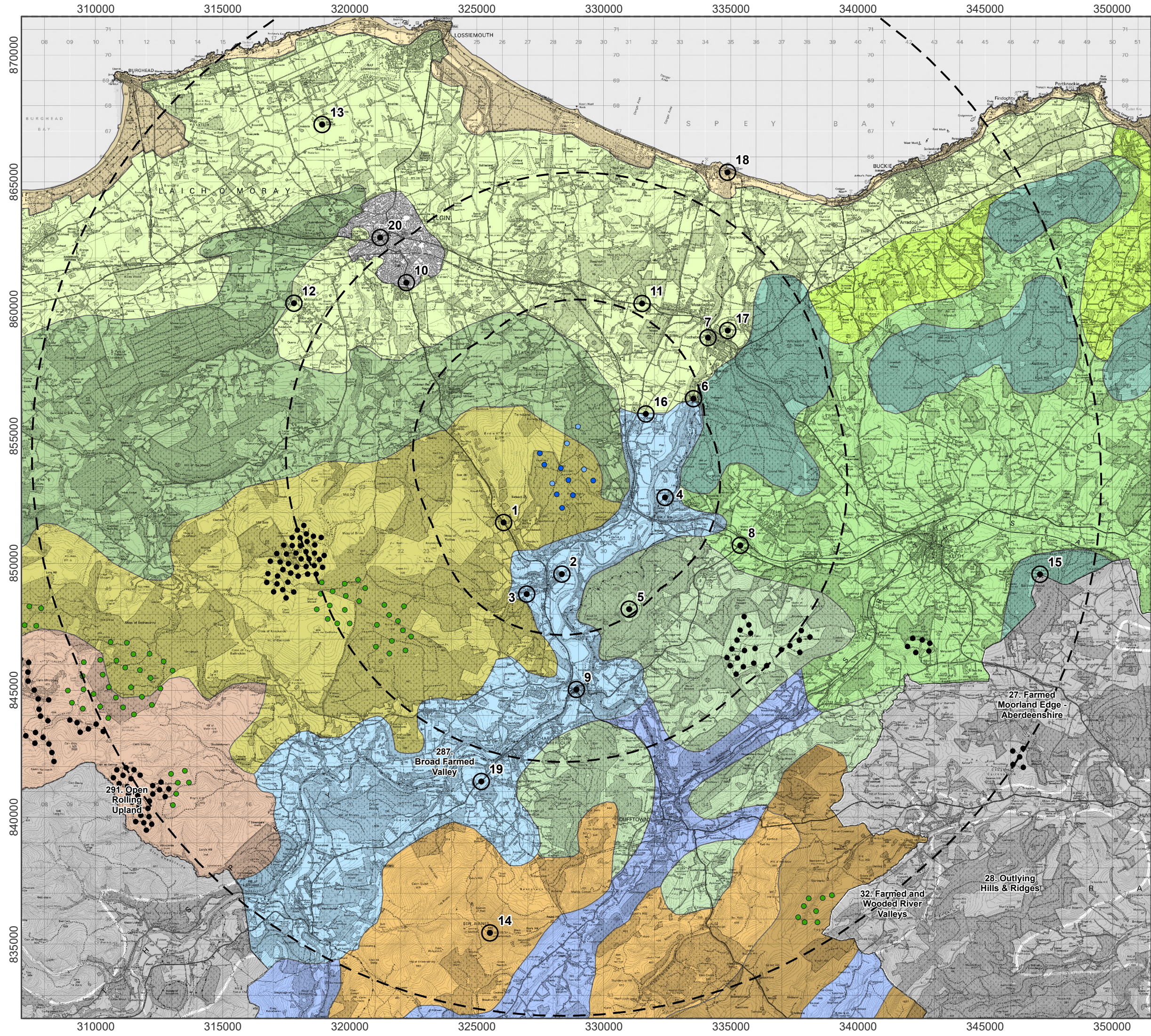
Figure 5.4: Landscape Character
