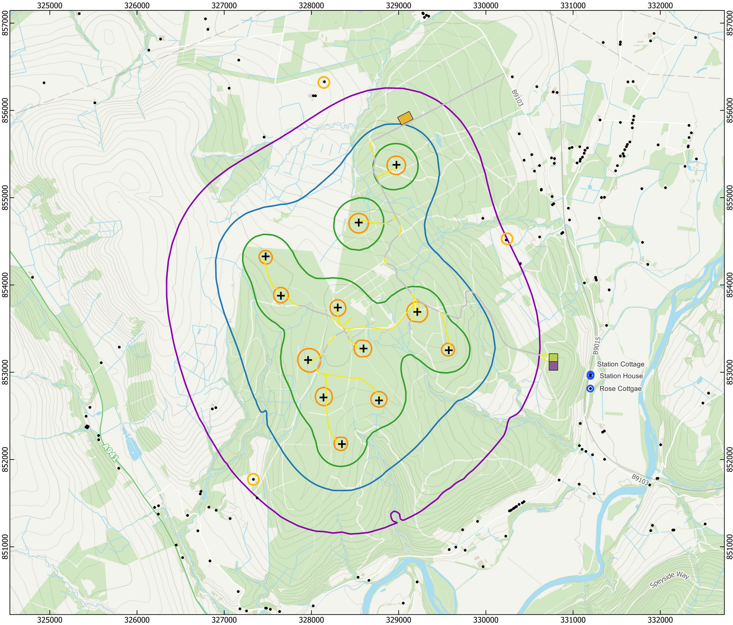
Figure 9.1 Noise Contour Plot
