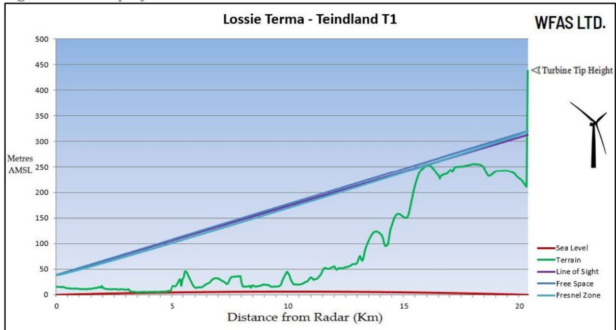
Figure 6 – radar projection RAF Lossiemouth TERMA
