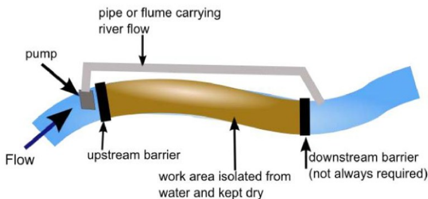
Plate 14: Typical over pumping arrangement 41
